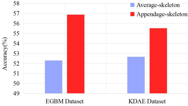
Fig. 6. Effects of appendage-based partitioning on recognition accuracy. In the ALR module, the influence of labels generated by different skeleton data partitioning on the ability of the final encoder to extract emotional representation.
